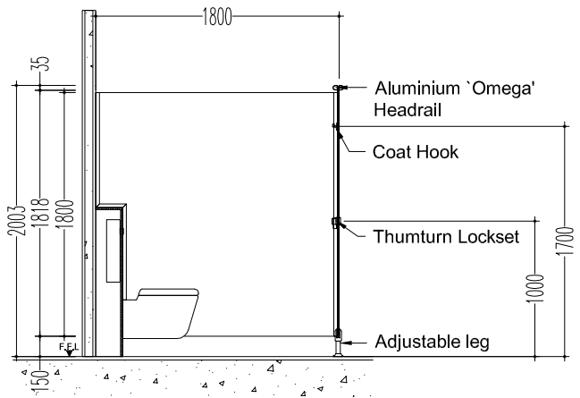
Section A
