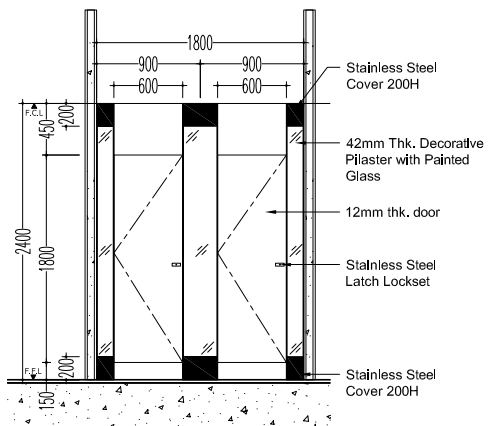
Front Elevation A
